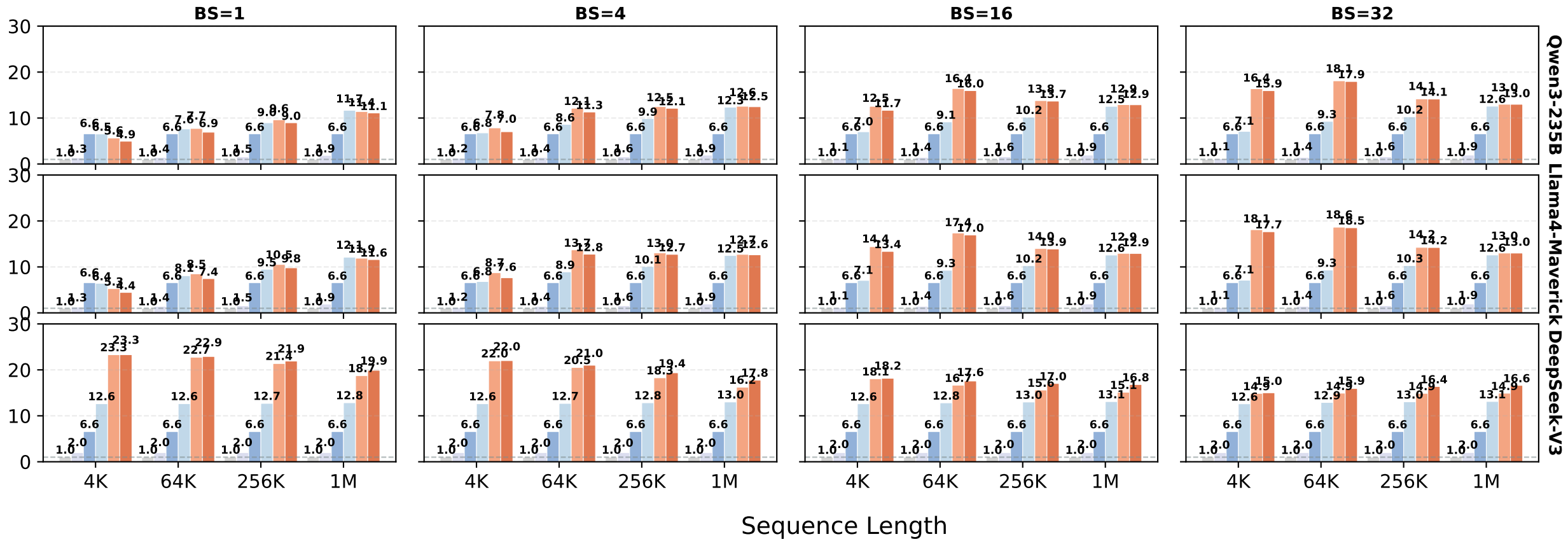
Latency Speedup
