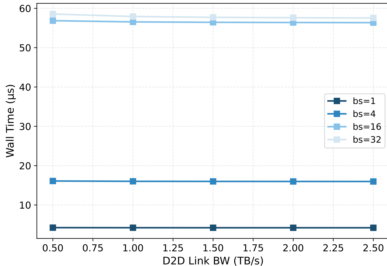
Wall Time vs D2D BW (96T)
