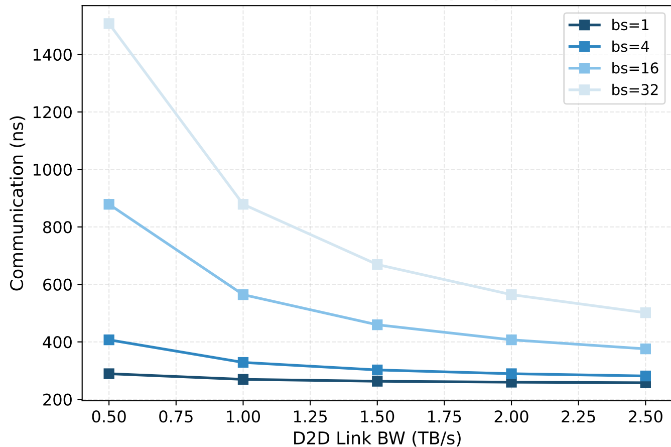
Comm vs D2D BW (96T)
