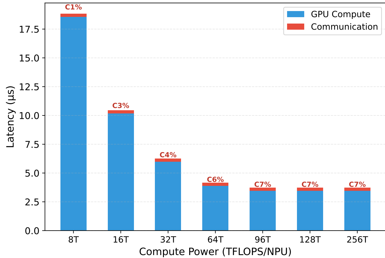
GPU vs Comm Breakdown (bs=1, D2D=1.5TB/s)
