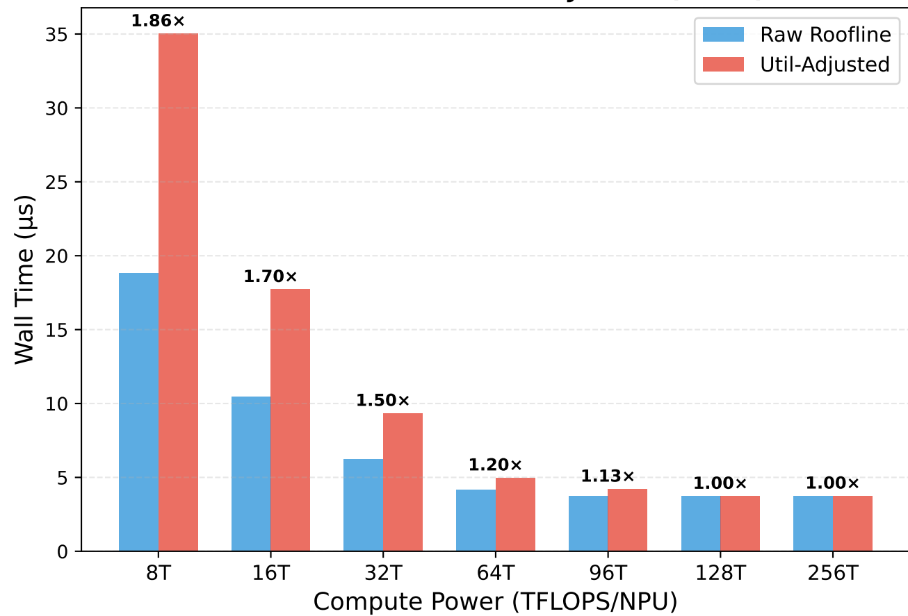
Raw Roofline vs Util-Adjusted (bs=1)
