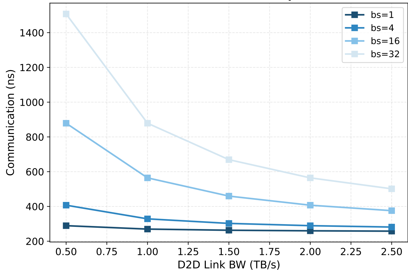
Comm Time vs D2D BW (Compute=96T)
