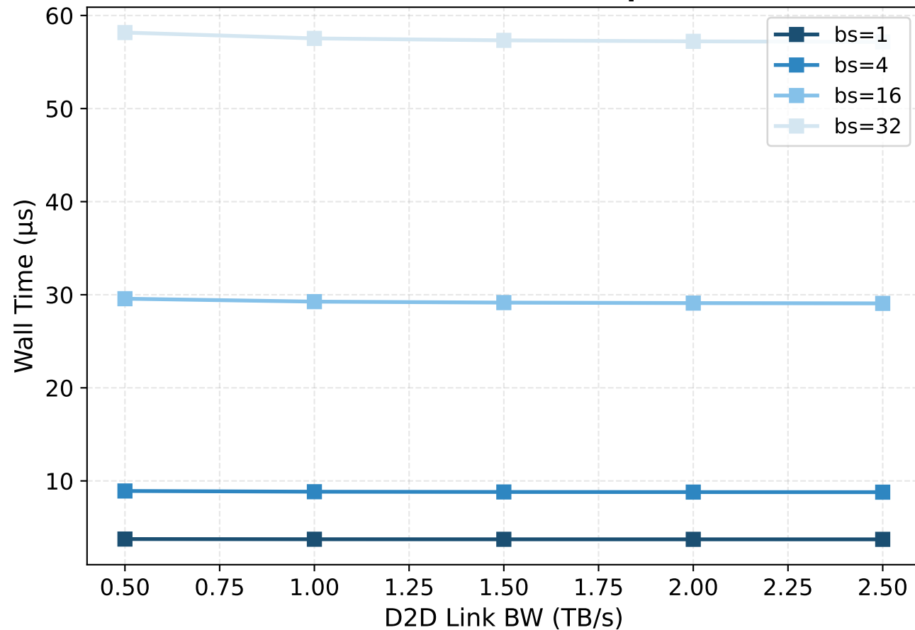
Wall Time vs D2D BW (Compute=96T)
