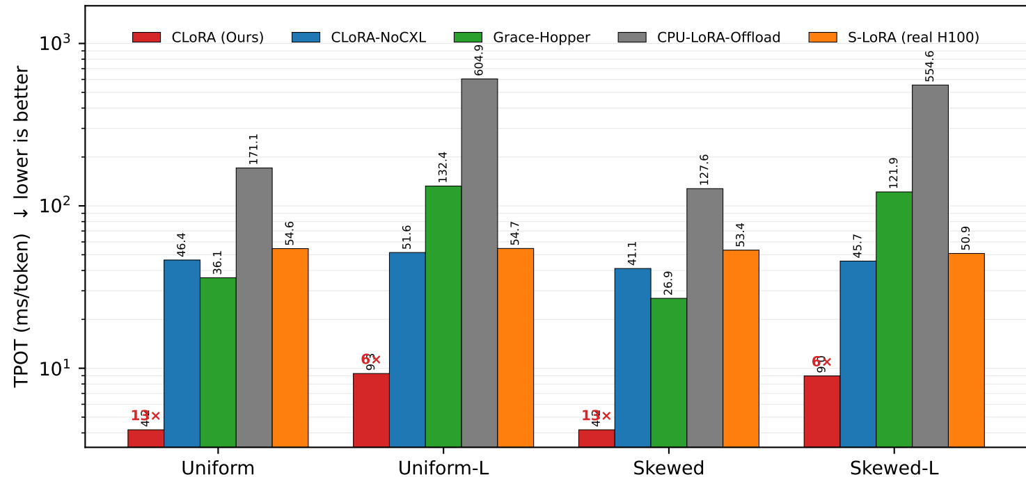
Llama2-7B decode, H100 — CLoRA & baselines (simulated) vs S-LoRA (real) CLoRA is 6-13 \times lower TPOT than measured S-LoRA
