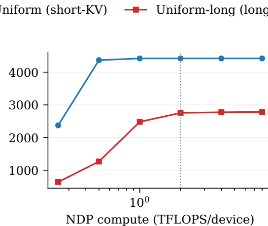
(c) NDP core throughput
