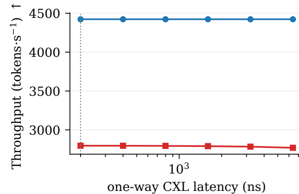
(a) CXL link latency
