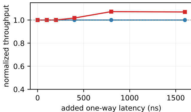
(c) NDP core throughput
