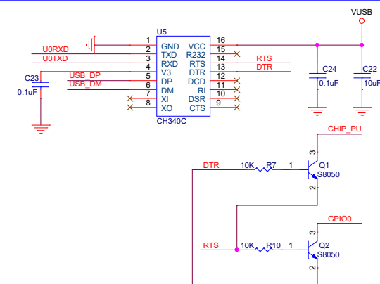
USB TO TTL
