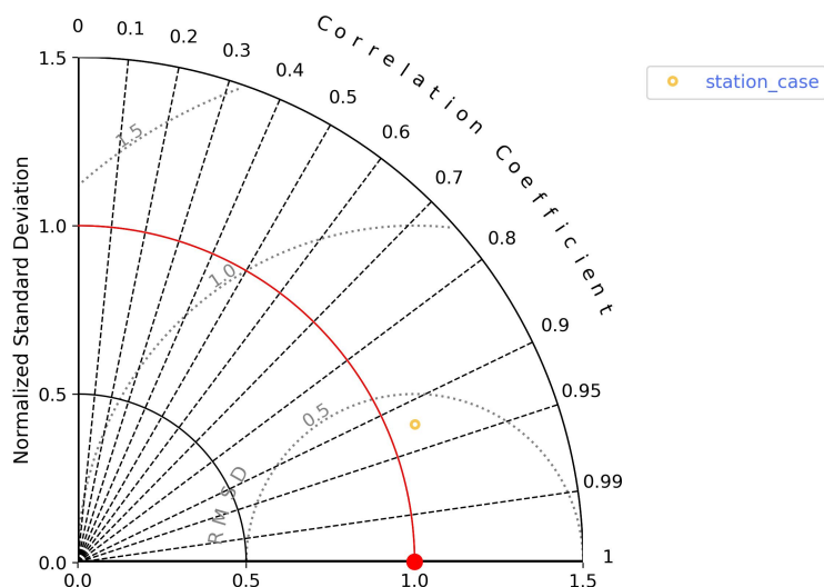
Figure 6: Taylor diagram for Latent_Heat against PLUMBER2 ( Taylor_Diagram_Latent_Heat_..._PLUMBER2.jpg ).
