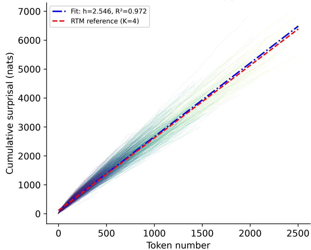
(a) LLM cross-entropy
