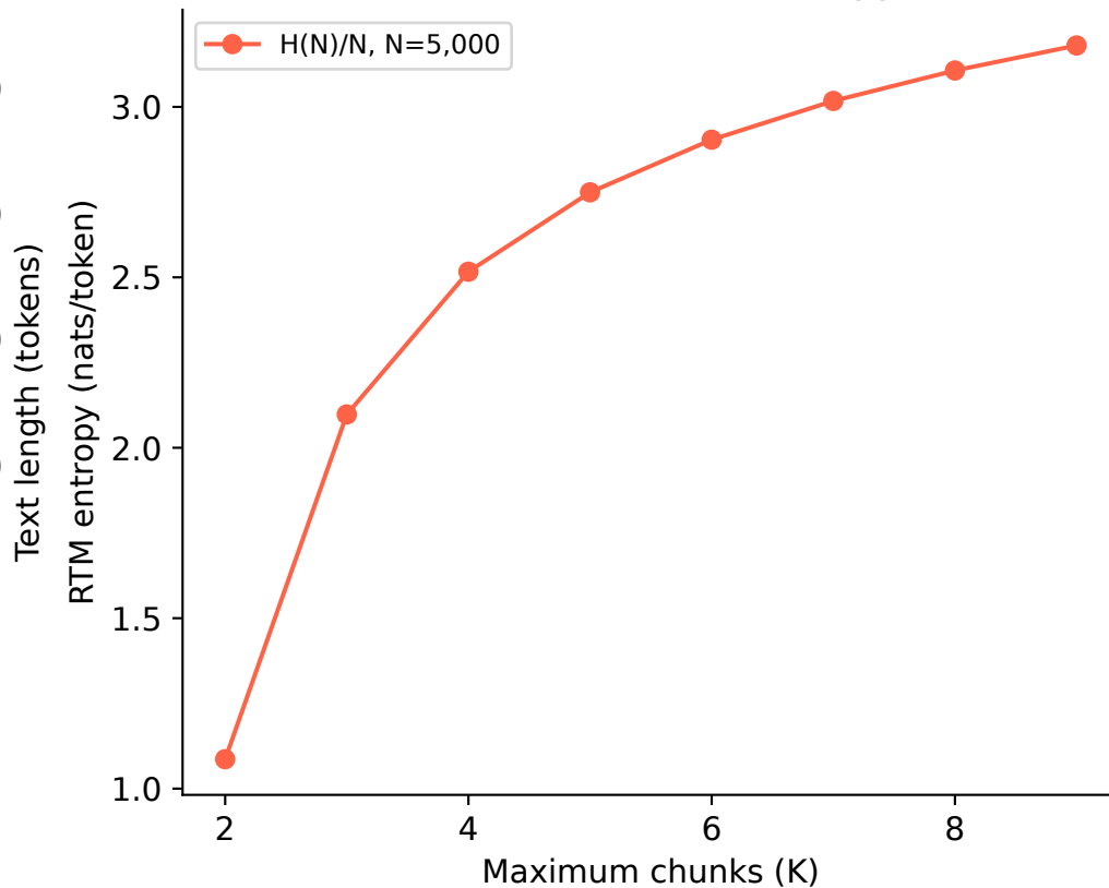
(b) Semantic-tree entropy
