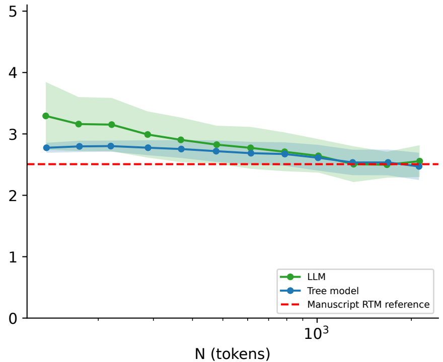
(c) Mean and standard deviation
