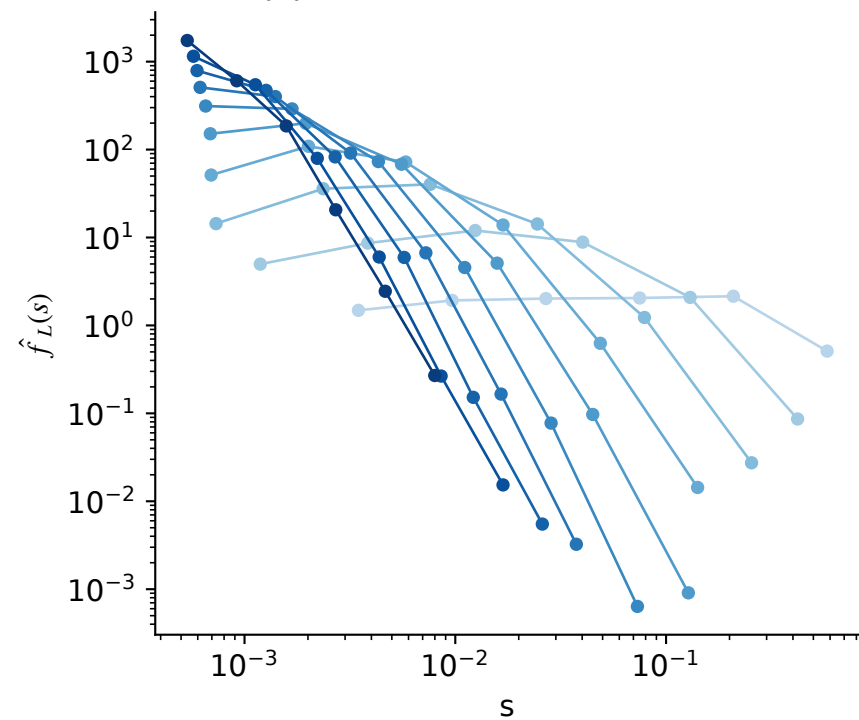
(c) 925-tree chunk densities
