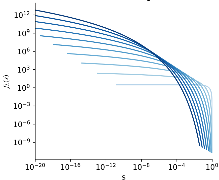
(c) 925-tree chunk densities
