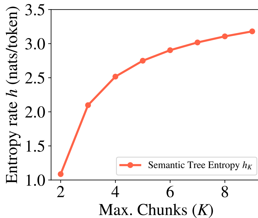
(b) Semantic Tree Entropy
