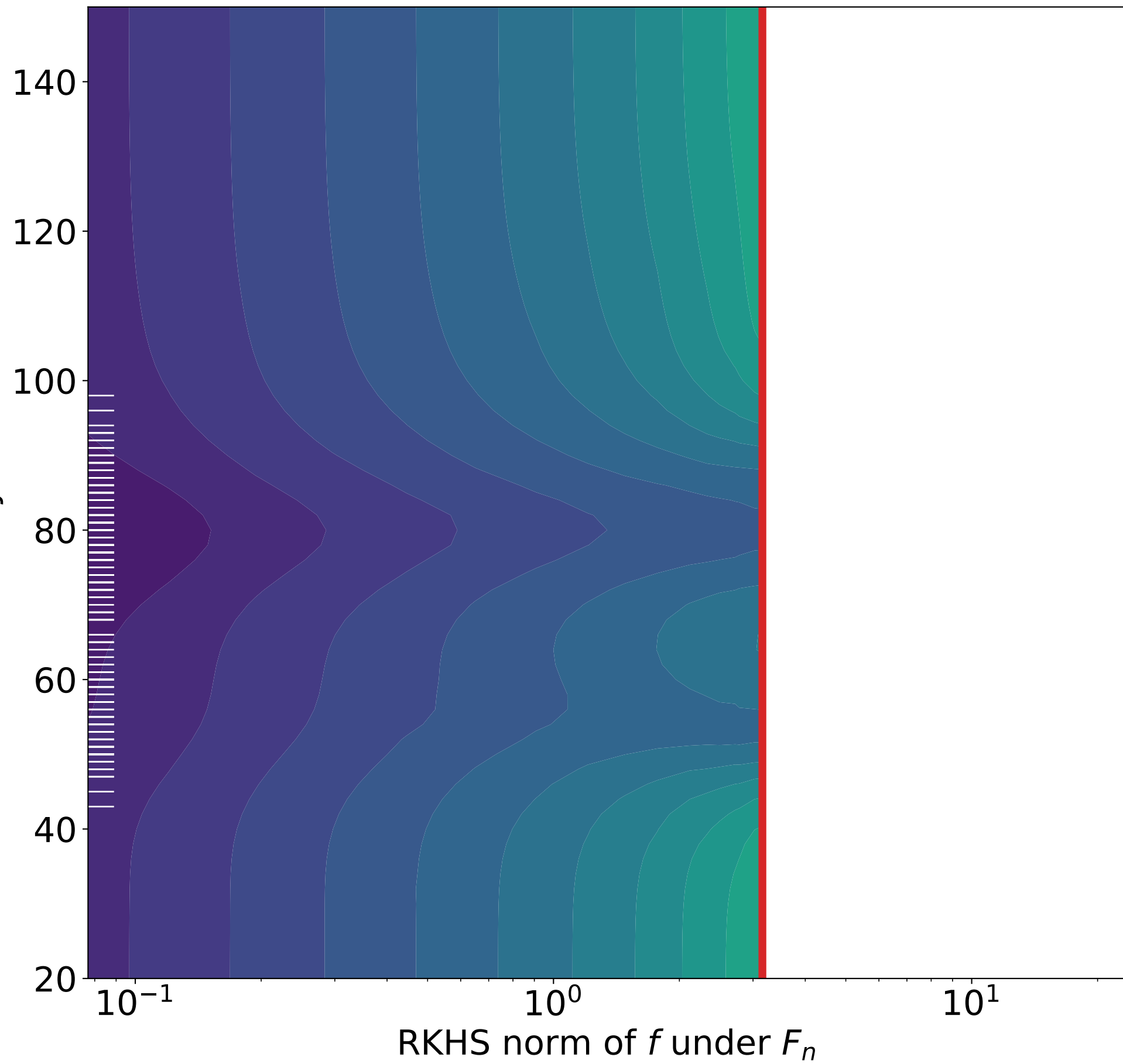
Maximum Likelihood
