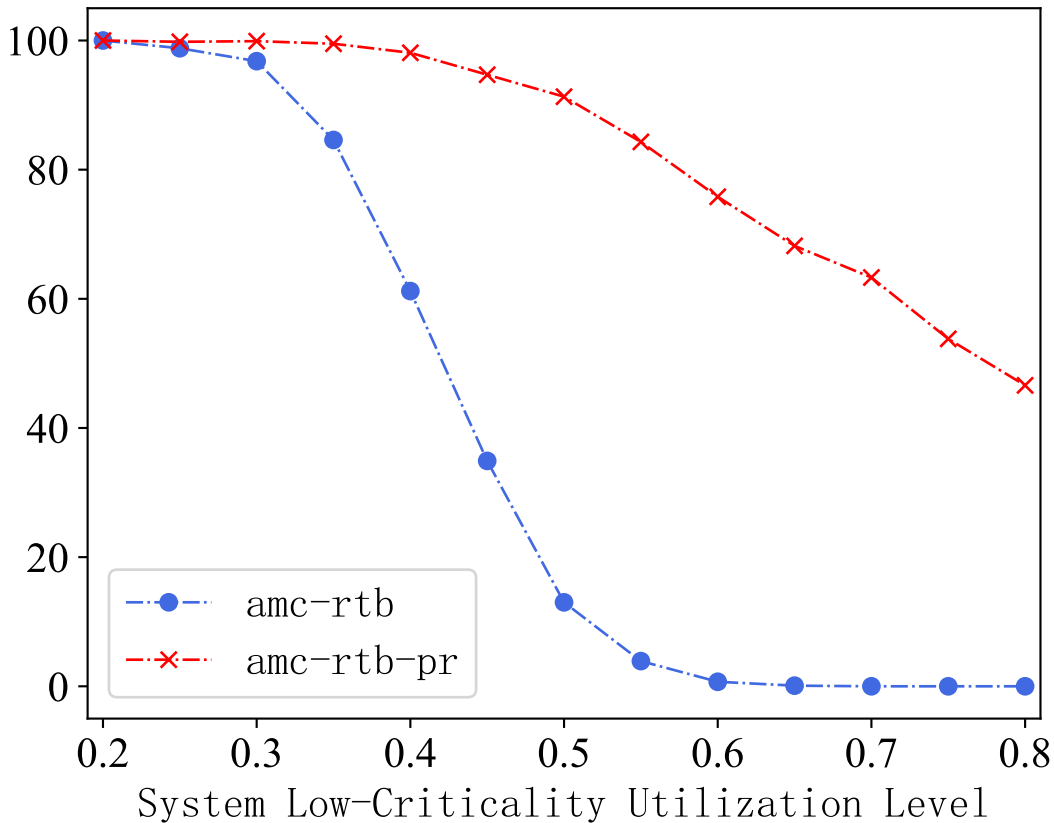
Task Schedulability Ratio
