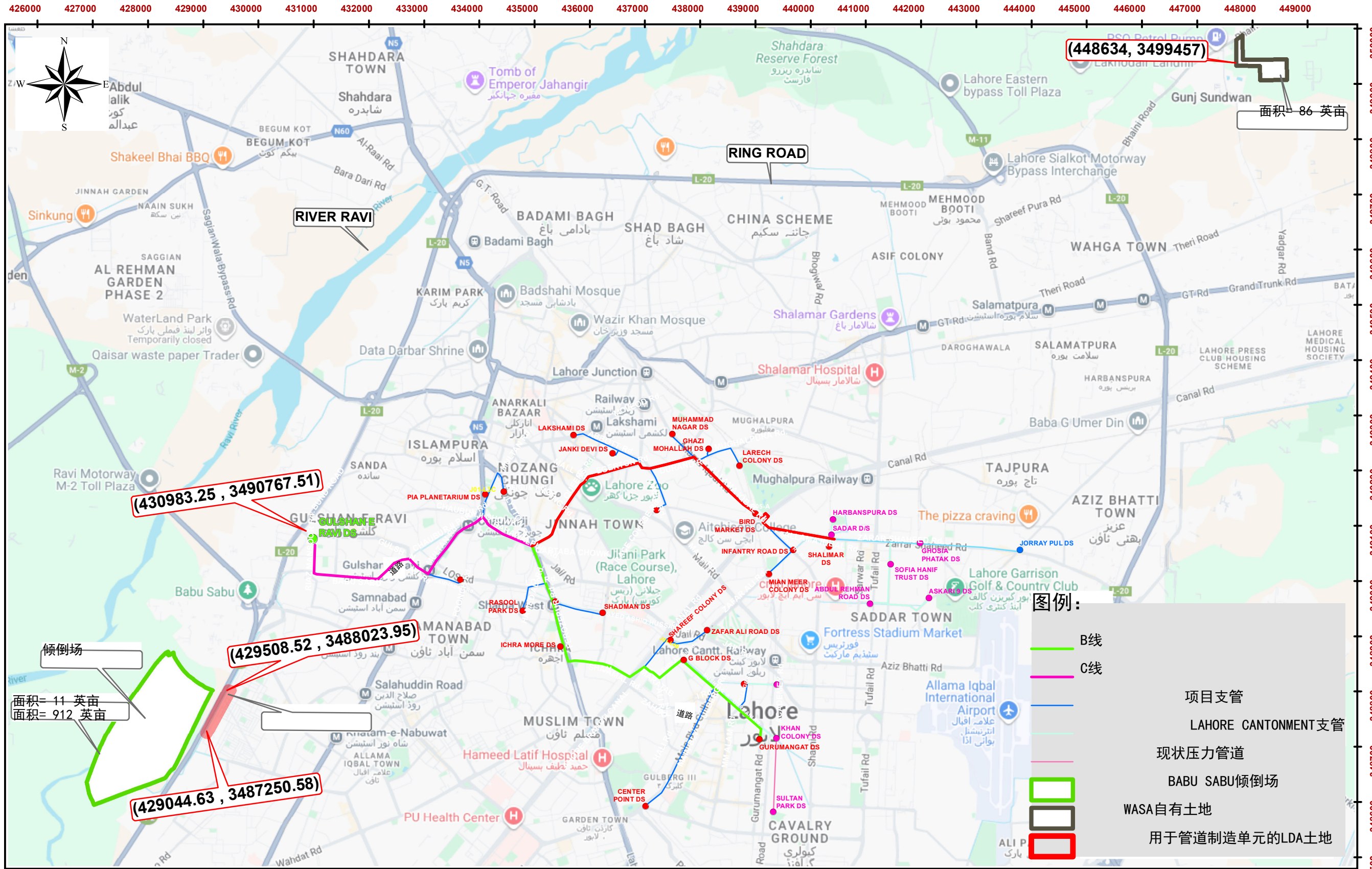
LAHORE WASTEWATER AND DRAINAGE MANAGEMENT PROJECT (LWDM) - 从LARECHS COLONY至GULSHAN-E-RAVI、LAHORE的污水管网（采用非开挖技术）
