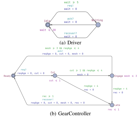
Fig. 1. Simplified gear-shift example.
