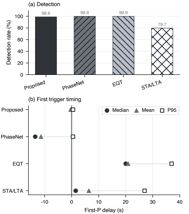
Fig. 3. First-P streaming latency comparison for CausalStreamingPPicker, PhaseNet, EQTransformer, and STA/LTA. The public window pickers are replayed with history-buffer-aligned native windows, so the comparison reflects first-trigger behavior under their public fixed-window interfaces.
