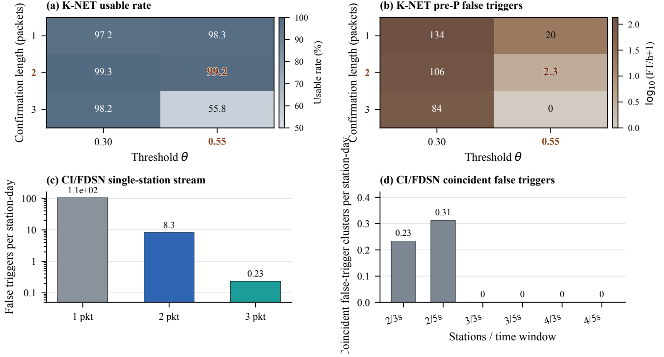
Fig. 7. Operating-point and continuous-stream evidence. Panels (a) and (b) show K-NET event usable rate and pseudo-continuous pre-P false-trigger episodes per hour across threshold and confirmation length; bold numbers mark \theta = 0.55 with two-packet confirmation. Panel (c) shows CI/FDSN continuous strong-motion single-station false triggers per station-day at \theta = 0.55 . Panel (d) shows coincident false-trigger clusters formed by different stations within short windows after two-packet station false triggers; zero clusters for three or more stations indicates that this event-free replay produced no network-level false-alert candidate meeting a three-station condition.
