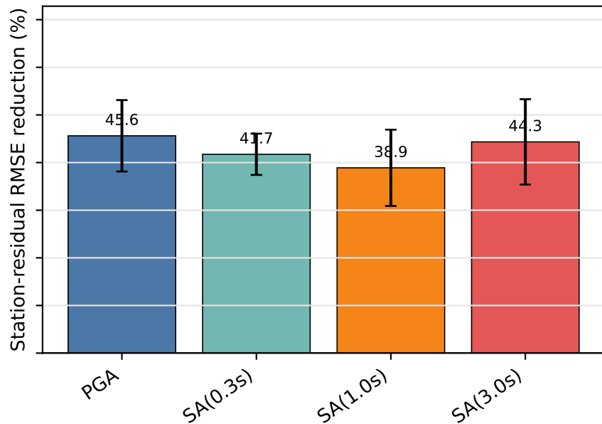
Spatial-block holdout
