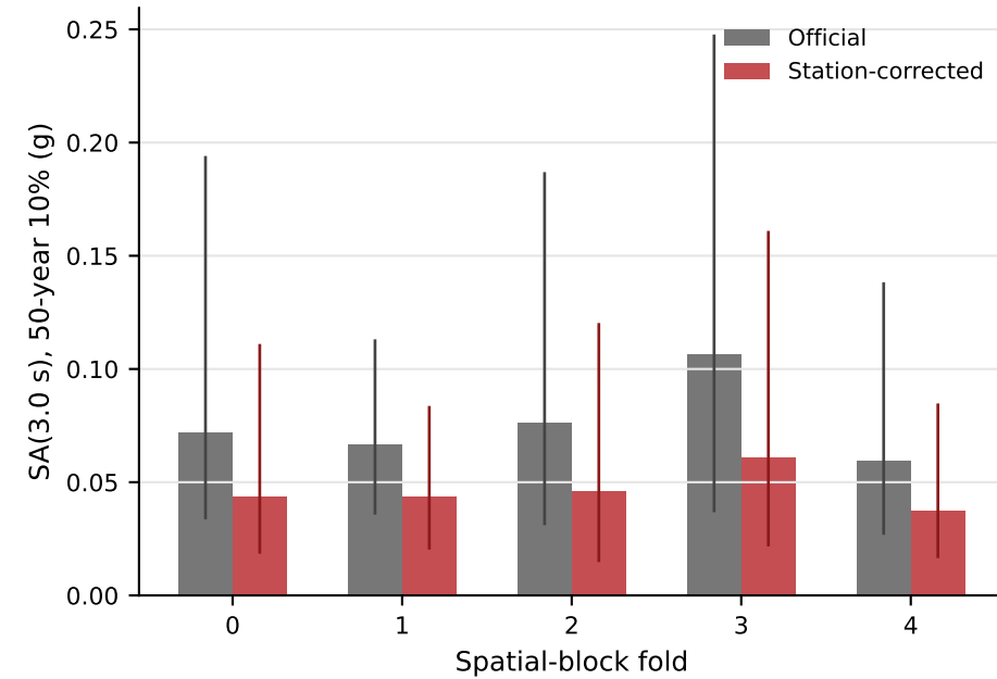
B Spatial-block fold medians
