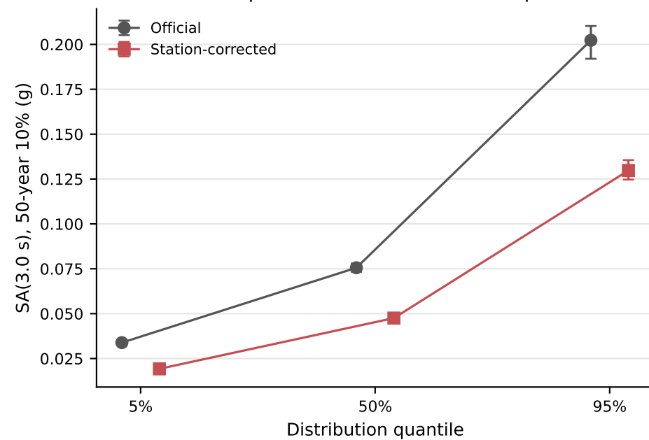
D Bootstrap intervals for distribution quantiles
