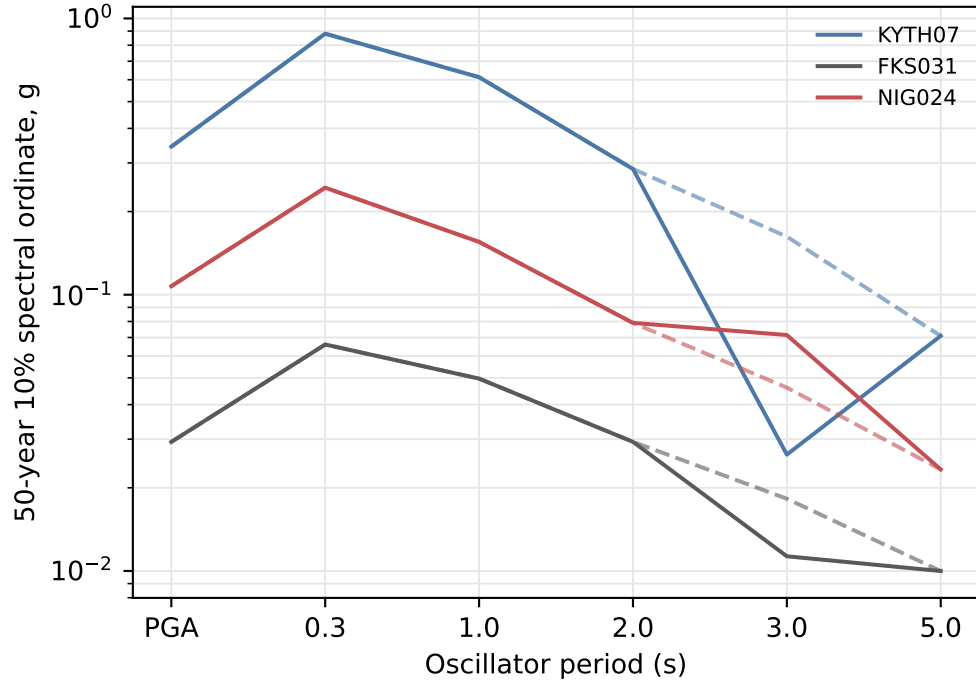
B UHS with only SA(3.0\text{ s}) shifted
