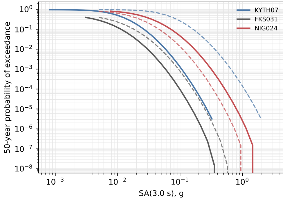
A OpenQuake SA(3.0 s) hazard curves
