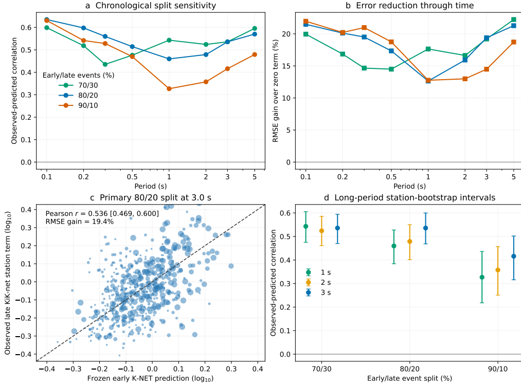
Supplementary Figure 11. Chronological cross-network station-field validation. a , K-NET-to-KiK-net correlations for fixed early/late event splits. b , root mean squared error reduction relative to a zero station term. c , frozen predictions from the earliest 80% of K-NET events against KiK-net terms estimated from the latest 20% at 3.0 s. d , station-bootstrap 95% intervals at 1–3 s. The reverse direction is reported in Supplementary Table 20.
