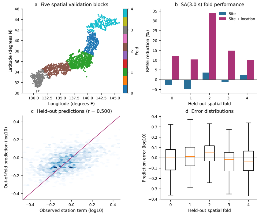
Supplementary Figure 4. Spatial validation of SA(3.0 s) station prediction. a , five station blocks used for cross-validation. b , root mean squared error reduction in each held-out block for the site-only and site-plus-location models. c , observed event-adjusted station terms and out-of-fold site-plus-location predictions. d , prediction-error distributions by spatial fold; boxes show interquartile ranges and whiskers extend to 1.5 times the interquartile range.
