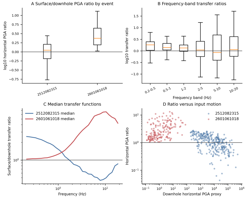
Supplementary Figure 10. KiK-net surface and downhole waveform comparison. a , horizontal surface-to-downhole peak acceleration ratios by earthquake. b , frequency-band Fourier amplitude ratios. c , median transfer functions for the two event sets. d , horizontal peak acceleration ratio against the downhole input-motion proxy. Ratios are shown in \log_{10} units in panels a and b .
