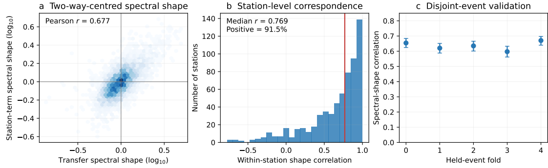
Supplementary Figure 3. Paired-sensor spectral-shape validation. a , two-way-centred station-term and surface–borehole transfer shapes across eight periods. b , distribution of within-station shape correlations. c , correlations when transfer spectra and station-term spectra are estimated from disjoint earthquake groups; bars are station-cluster bootstrap 95% intervals.
