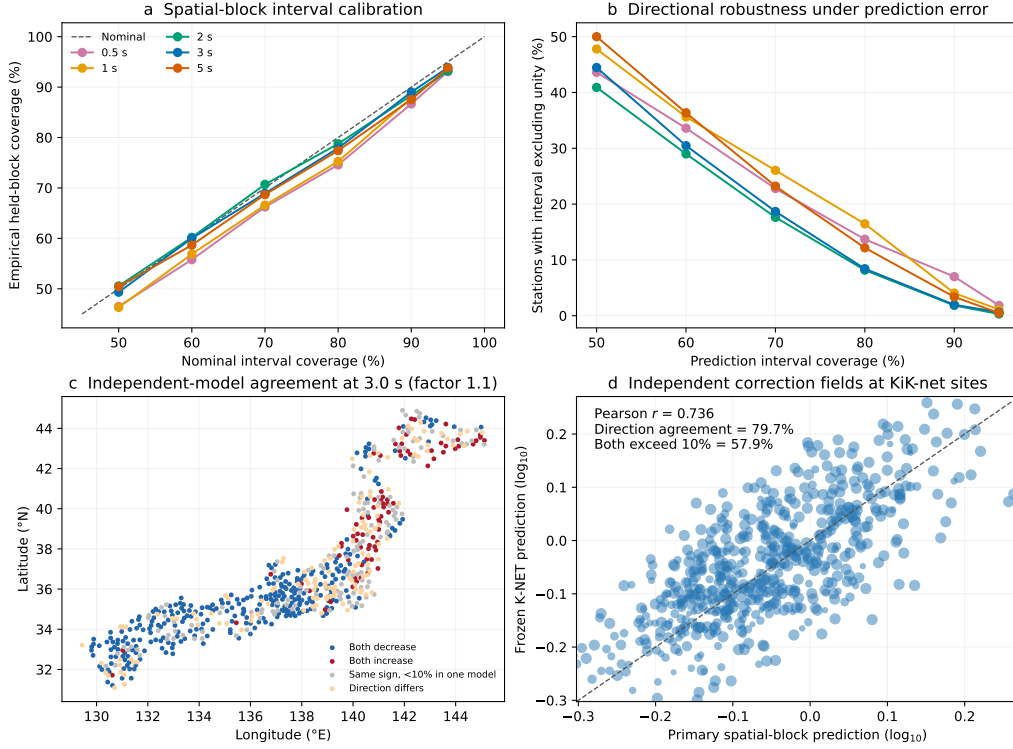
Supplementary Figure 9. Uncertainty and independent-model stability of station corrections. a , empirical spatial-block coverage against nominal coverage. b , fraction of station intervals excluding a unit multiplier. c , 3.0 s KiK-net sites classified by agreement between the primary and frozen K-NET correction fields. d , the two independent correction fields at 3.0 s. Prediction intervals and model agreement quantify different uncertainty components.
