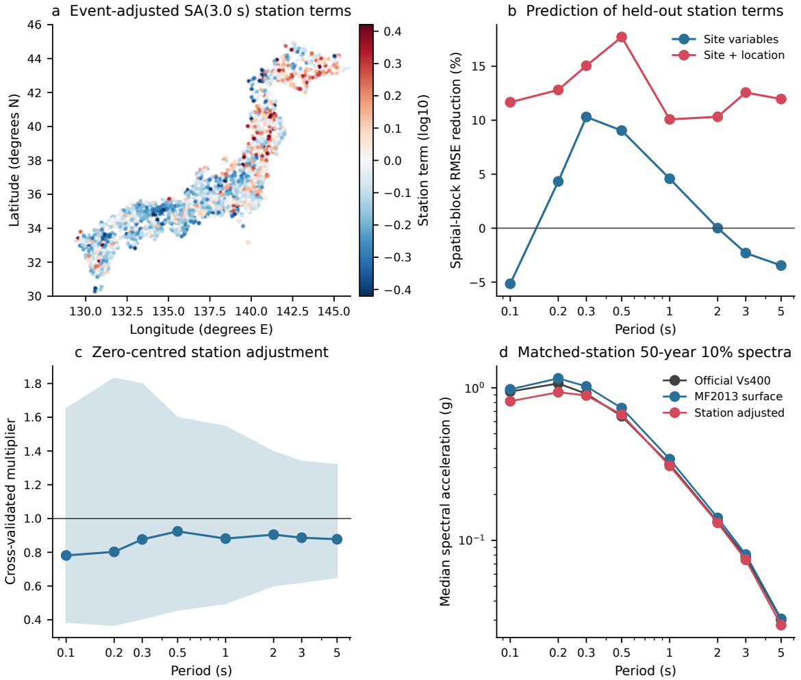
Figure 4. Primary full-sample prediction and response-spectrum propagation. a , event-adjusted SA(3.0 s) station terms at stations with at least 20 records. b , spatial-block root mean squared error reduction for models using site variables and site plus location variables. c , median and 5th–95th percentile range of zero-centred cross-validated station multipliers. d , matched-station median 50-year 10% response spectra on official V_S = 400 \text{ m s}^{-1} engineering bedrock, after projection to the station surface condition, and after the station adjustment. All periods are calculated directly.
