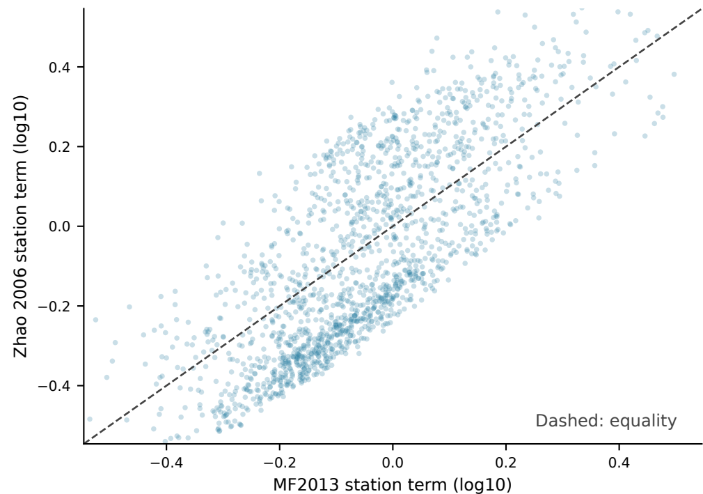
c Repeatability across earthquake groups
