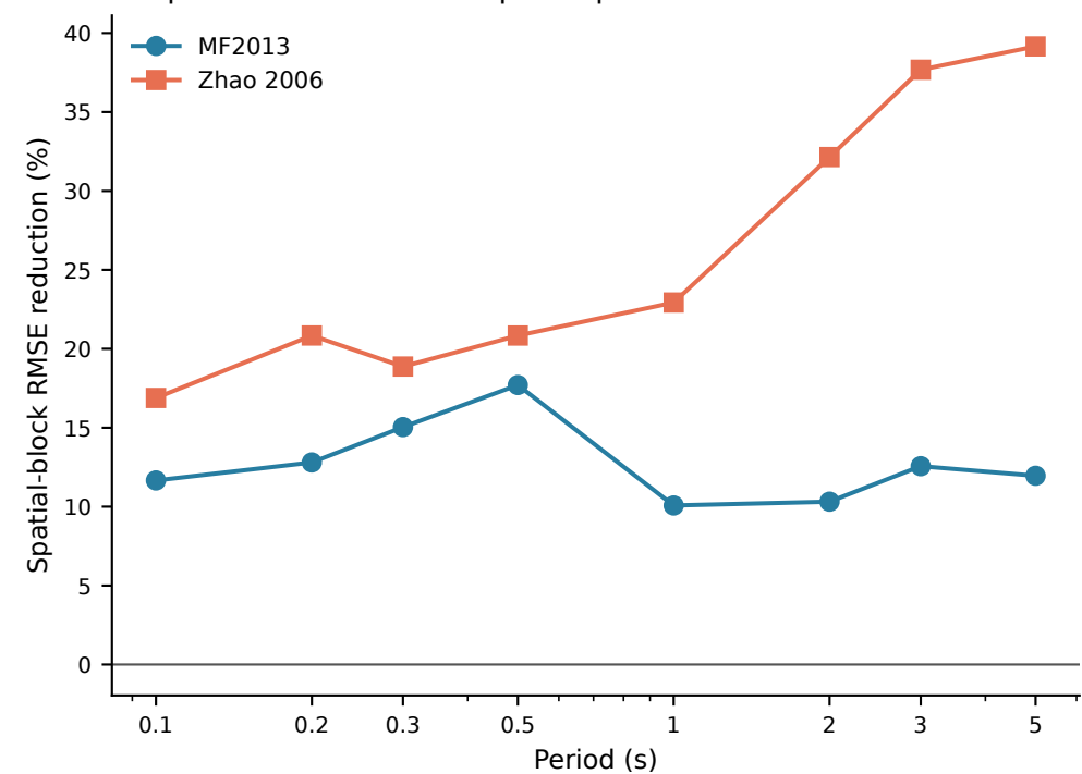
d Spatial estimation from public parameters
