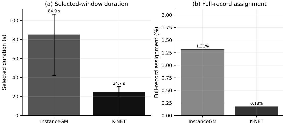
Figure 3: Selected-window duration and full-record assignment rate for the shortest-stable rule. The rule chooses longer typical windows for InstanceGM and shorter typical windows for K-NET. Only a small fraction of records are assigned to the full interval under the default PGA-retention and energy-retention criteria.
