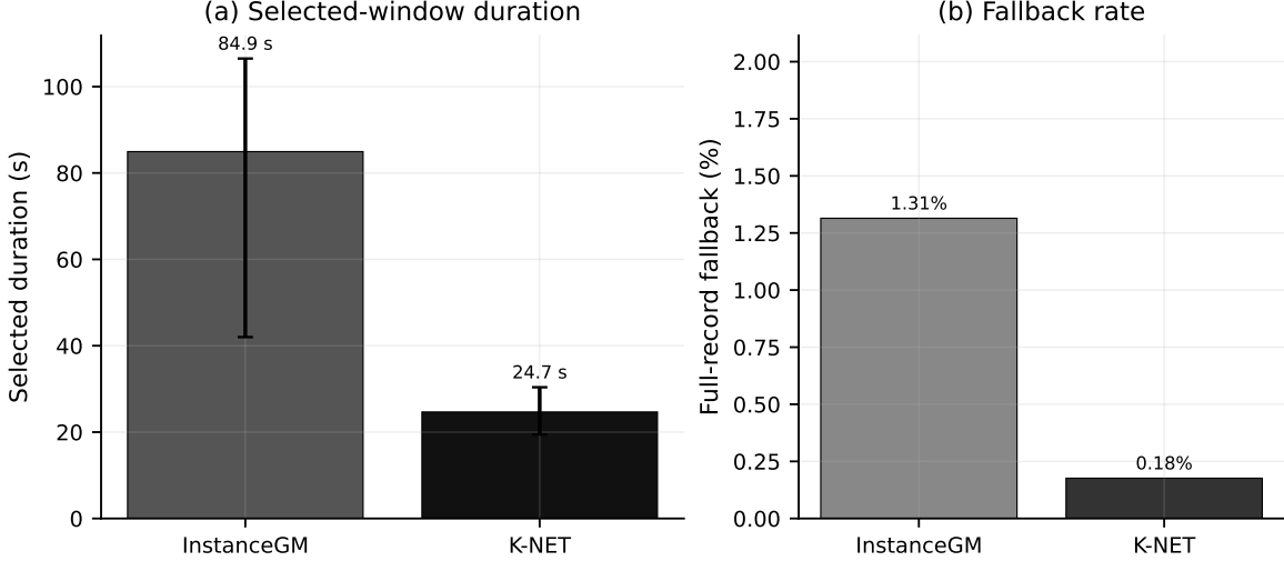
Figure 3: Selected-window duration and full-record fallback rate for the shortest-stable selector. The selector chooses longer typical windows for InstanceGM and shorter typical windows for K-NET. Full-record fallback remains low at the default PGA-retention and energy-retention criteria.
