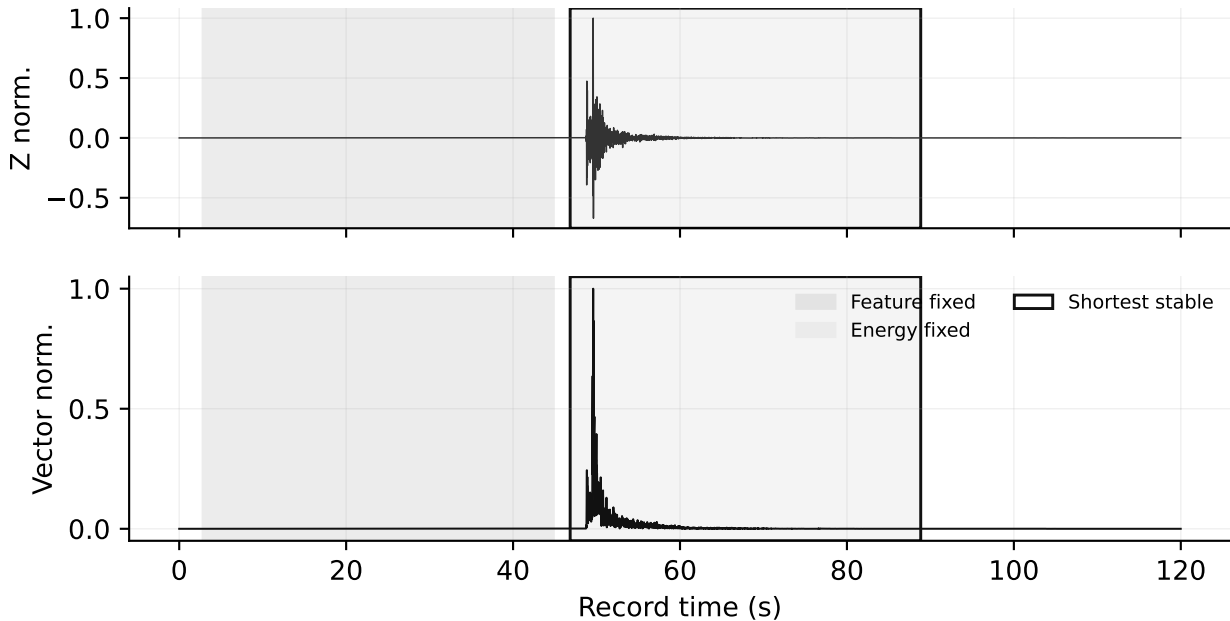
case_01 | InstanceGM | low magnitude | M1.9 | InstanceGM fixed-window failure
