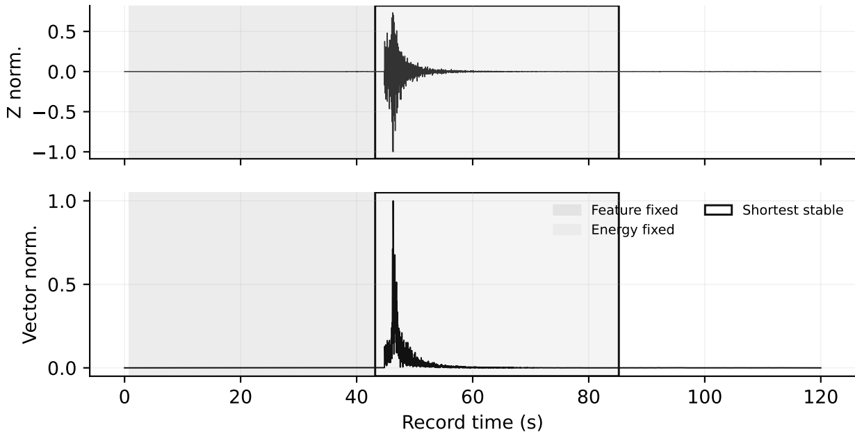
case_02 | InstanceGM | low magnitude | M2.1 | InstanceGM fixed-window failure
