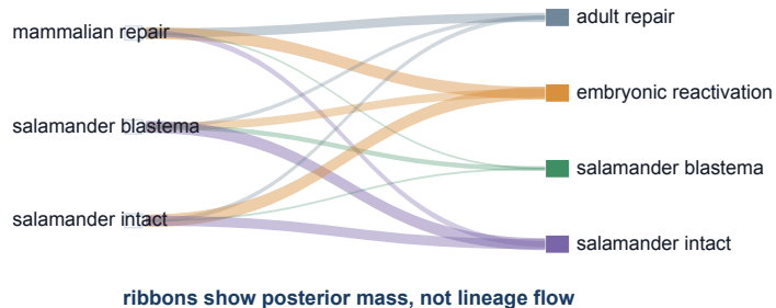
b Observed-group to latent-regime posterior allocation
