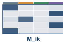
matrix and local transition representation
