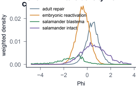
c One Phi mixture-density view
