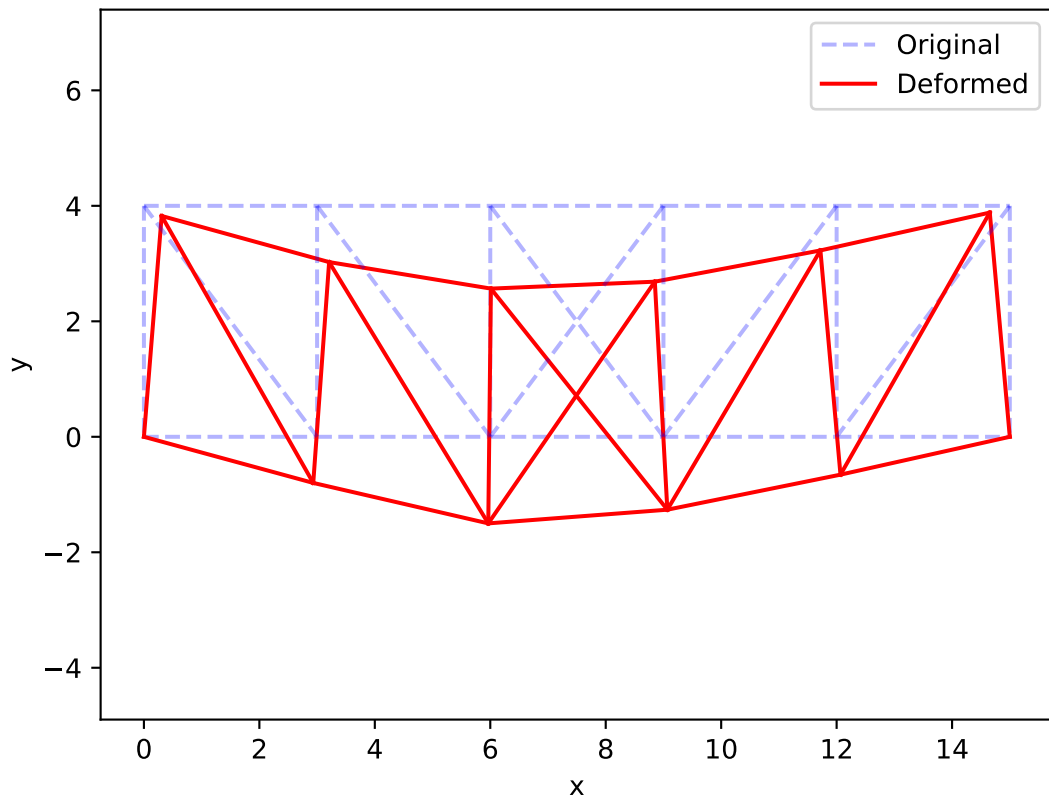
Deformed Truss (Scale: 15673.0x)
