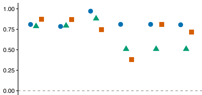
Prediction merge
