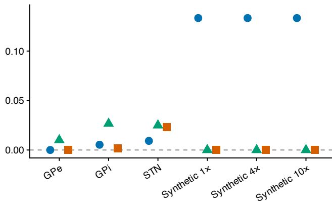
Reference-event fragmentation
