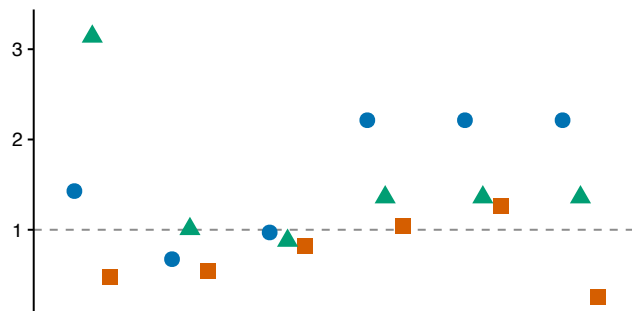
Reference-event fragmentation
