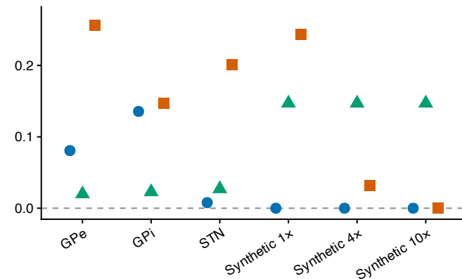
Prediction merge
