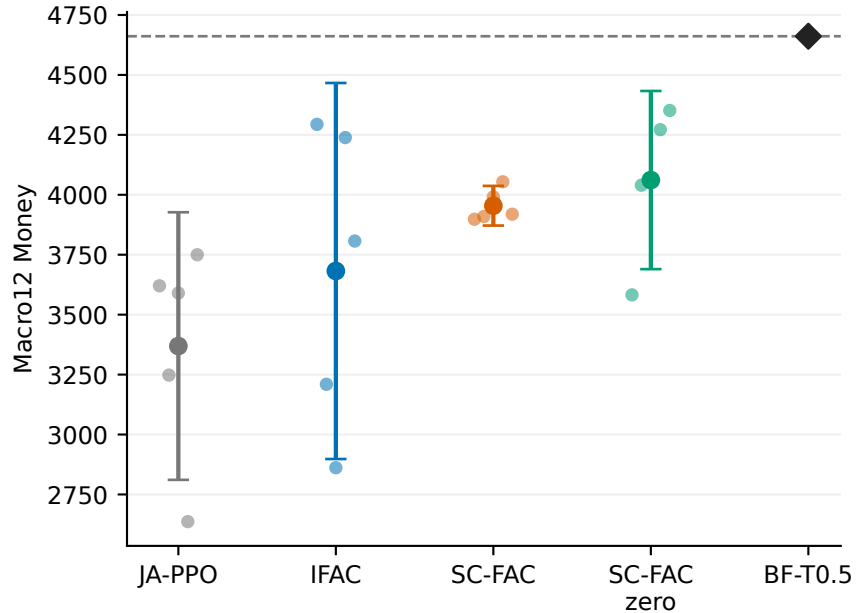
NEW12: five-seed means and marginal 95% t intervals
