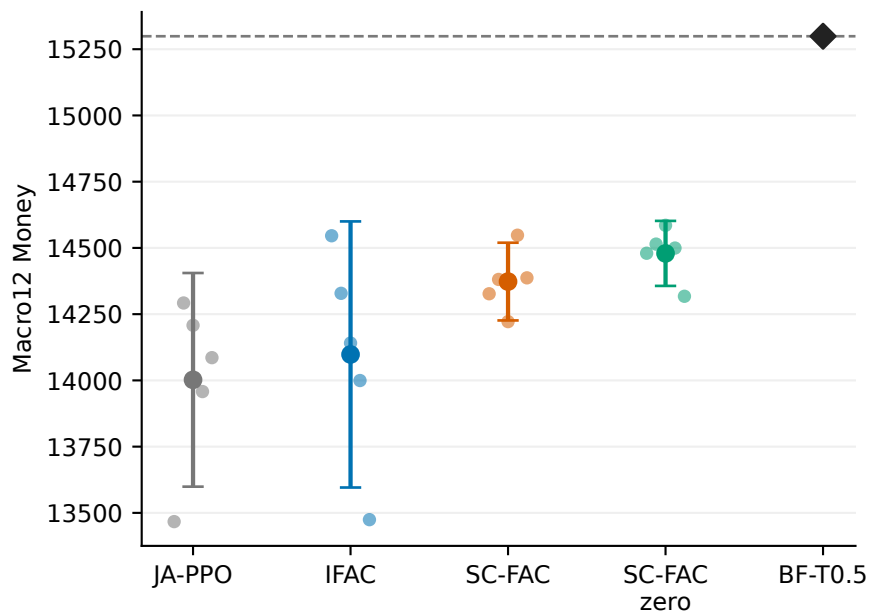
NEW12: five-seed means and marginal 95% t intervals
