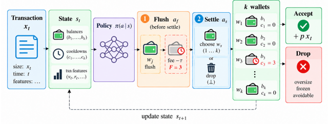
Fig. 1. One collateral-control decision. The policy selects a settle action and a flush action; the environment executes the flush first (fee \tau , cooldown F ) and settlement second. Accepted value earns p x_t ; drops are oversize, frozen, or avoidable (the binary availability indicator is not drawn in s_t ).
