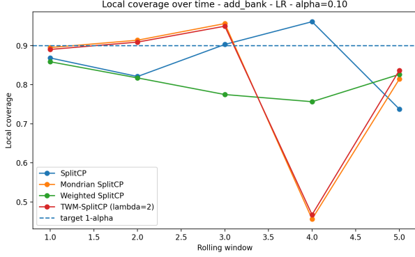
(c) Additional Bank, LR, local coverage at \alpha = 0.10 .
