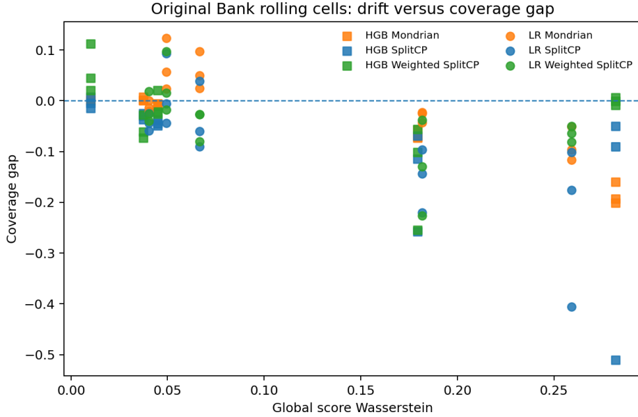
Figure 4: Original Bank rolling cells: global score Wasserstein versus coverage gap. Each point is one (method, window, \alpha ) cell, with marker shape indicating model and colour indicating method. Overall Pearson correlation between global score Wasserstein and coverage gap is r = -0.59 across all cells.
