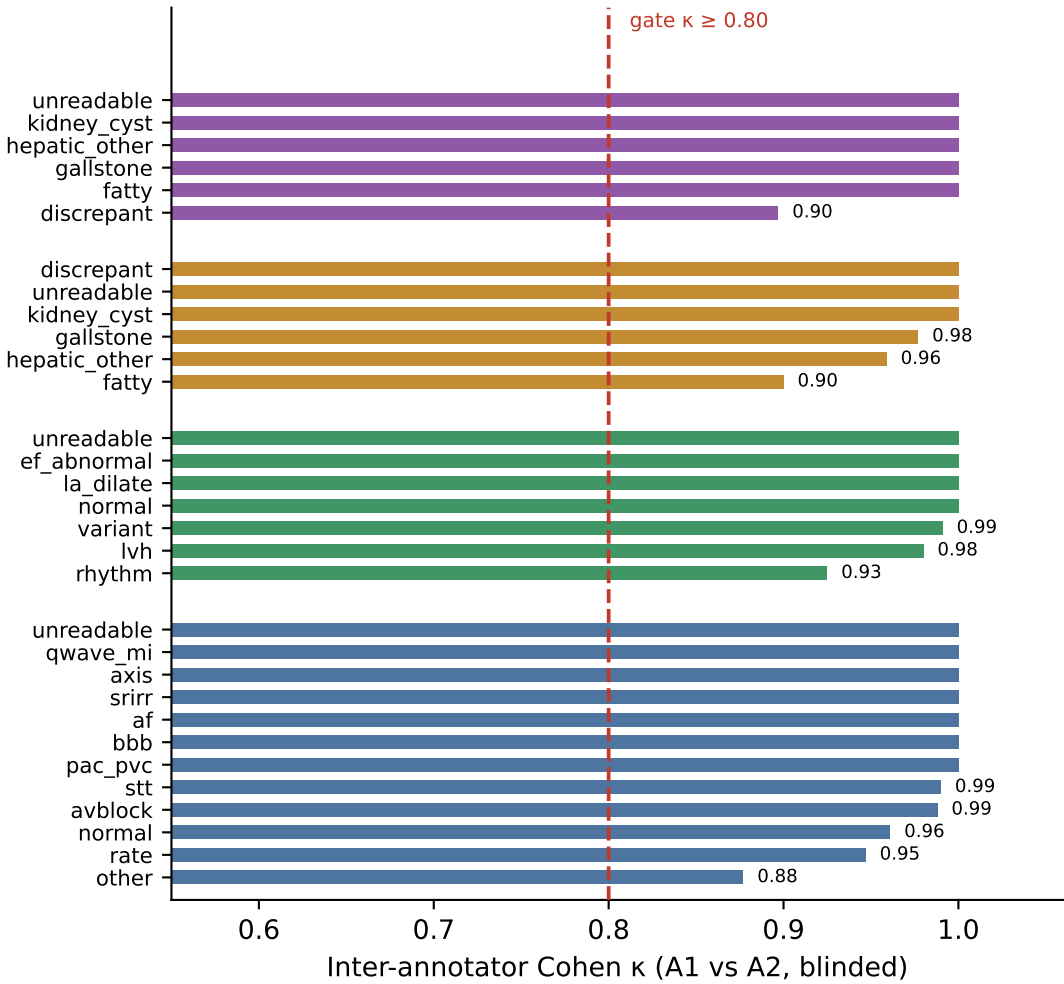
(b) 31/31 variables meet the \kappa \geq 0.80 gate (grouped by domain)
