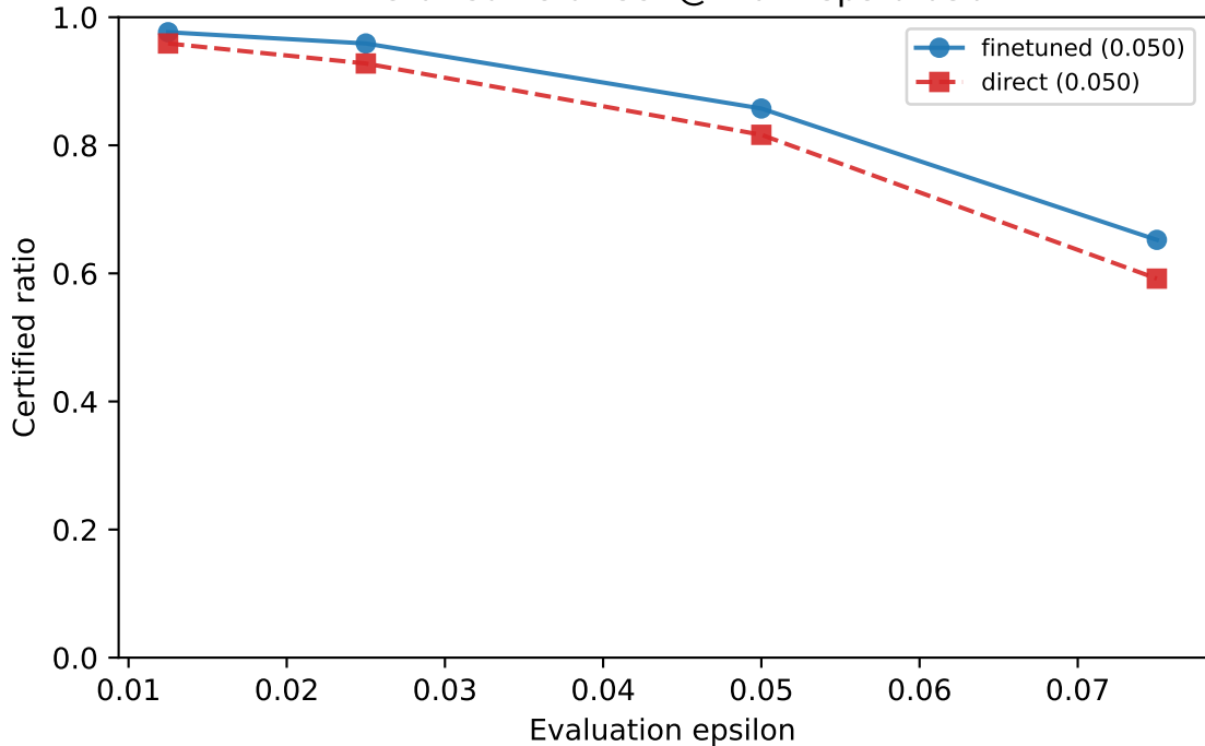
finetuned vs direct @ train eps 0.050
