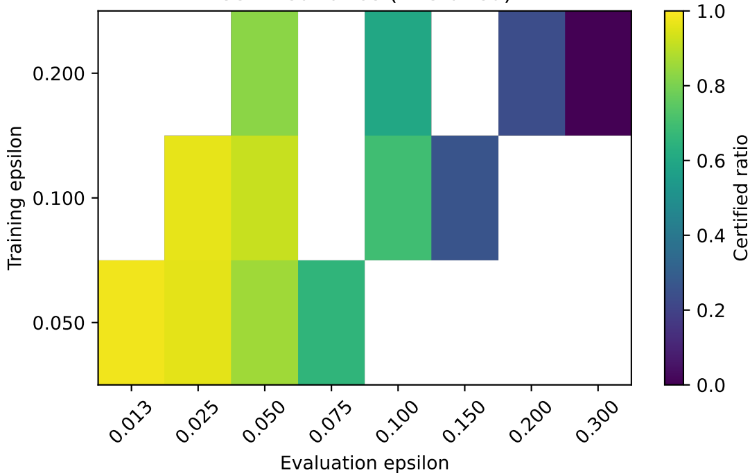
Certified ratios (finetuned)
