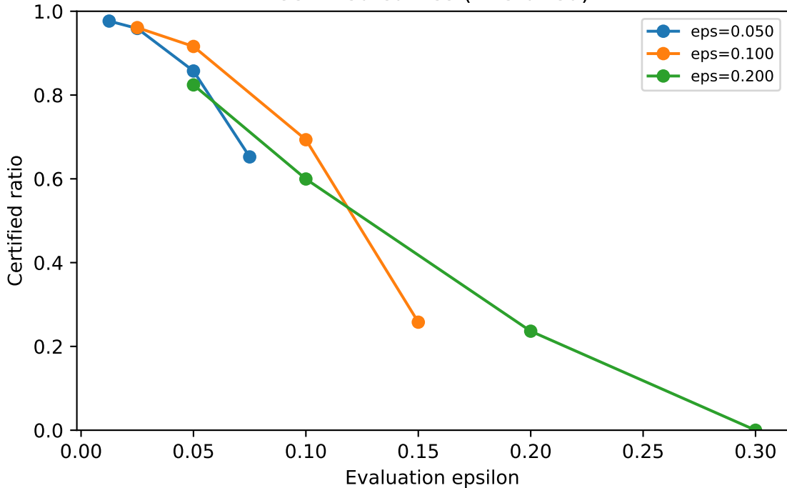
Certified curves (finetuned)
