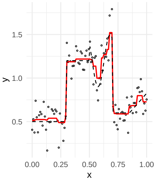
TV Denoising
