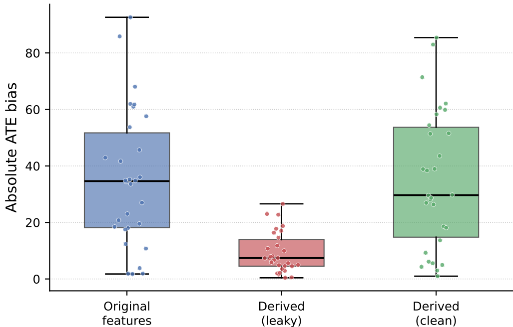
ATE bias over 30 independent seeds
