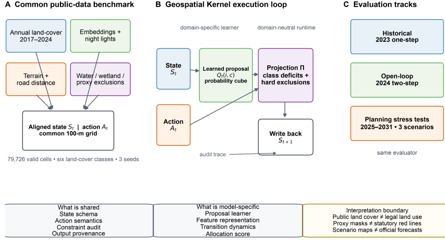
Figure 1 | Benchmark and Geospatial Kernel execution contract. Public annual land-cover, embedding, night-light, terrain and road layers are aligned to a common 100-m Abu Dhabi grid. Each model receives the same state, action and public proxy exclusions. The Geospatial Kernel exposes a learned proposal, constraint projection and state writeback. Historical, open-loop and planning tracks use one audit contract. The schematic does not imply statutory planning boundaries.
