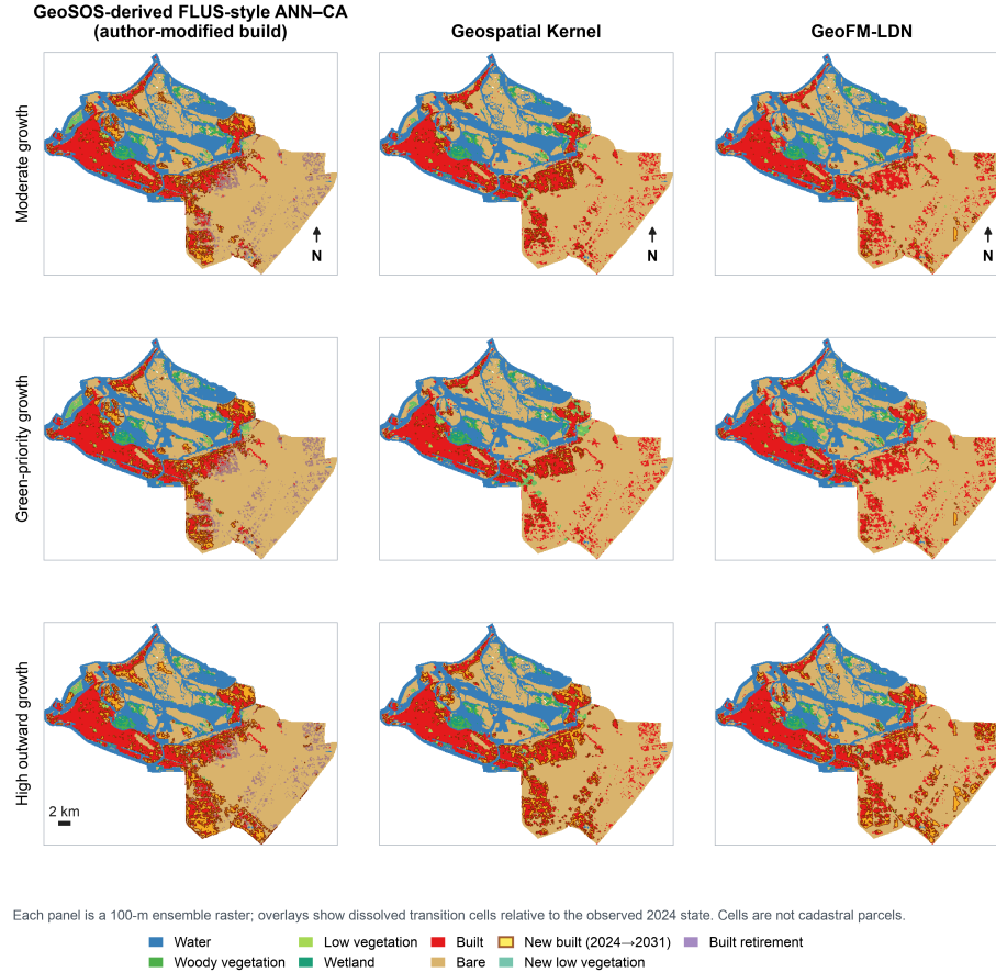
Figure 5 | 2031 spatial footprints. Each panel is a 100-m ensemble raster relative to the observed 2024 state. Overlays identify newly built, newly low-vegetated and retired-built cells; they are raster-cell change footprints, not cadastral parcels.
