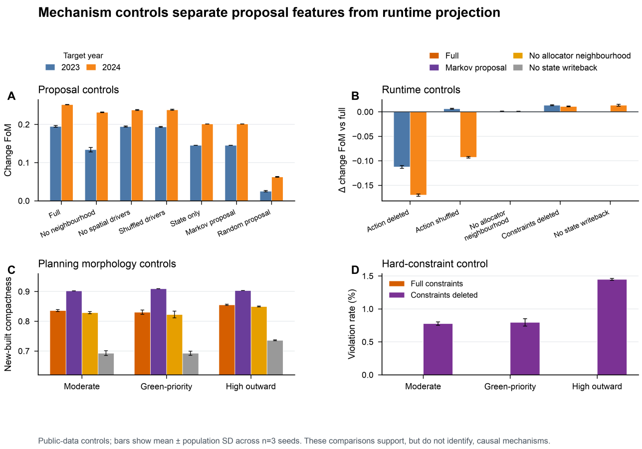
Figure 4 | Mechanism controls. Proposal, allocator, action, constraint and writeback controls are compared under the same public-data protocol. Deleting the action lowers historical strict FoM, whereas deleting the hard constraint raises agreement with noisy labels while violating the planning contract. These are diagnostic ablations, not causal policy experiments.
