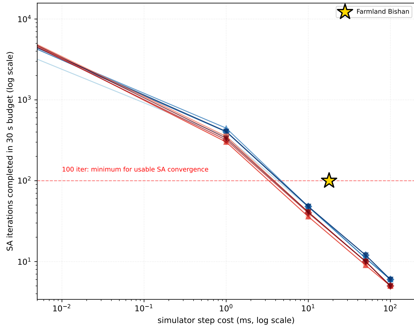
(b) Why SA wins/loses: search budget collapses with step cost
