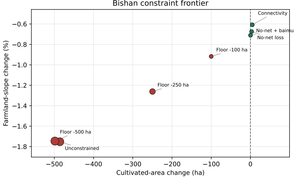
Figure S1: Bishan execution-constraint frontier. Points show independently recomputed farmland-slope change versus total cultivated-area change for the seven execution profiles in Table S19; marker area scales with the absolute qualifying baimu fang area change and colour distinguishes profiles that violate (red) or satisfy (green) cultivated-area no-net-loss. The dashed vertical line is the policy no-net-loss boundary.
