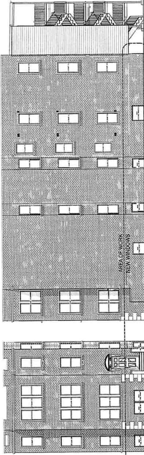
1 WEST ELEVATION 1/4" = 1'-0"
