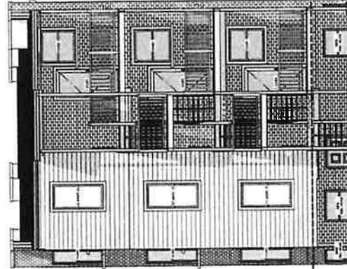
1 WEST ELEVATION 1/4" = 1'-0"
