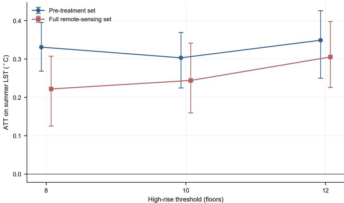
Threshold-placebo sensitivity in the Chongqing UHI case
