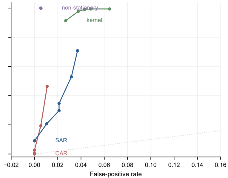
(b) Process-family ROC
