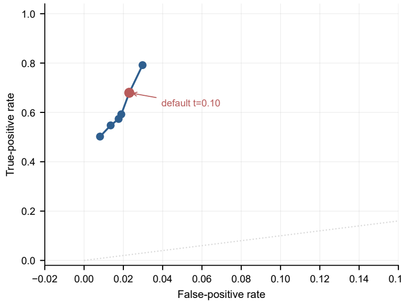
(a) Pooled ROC
