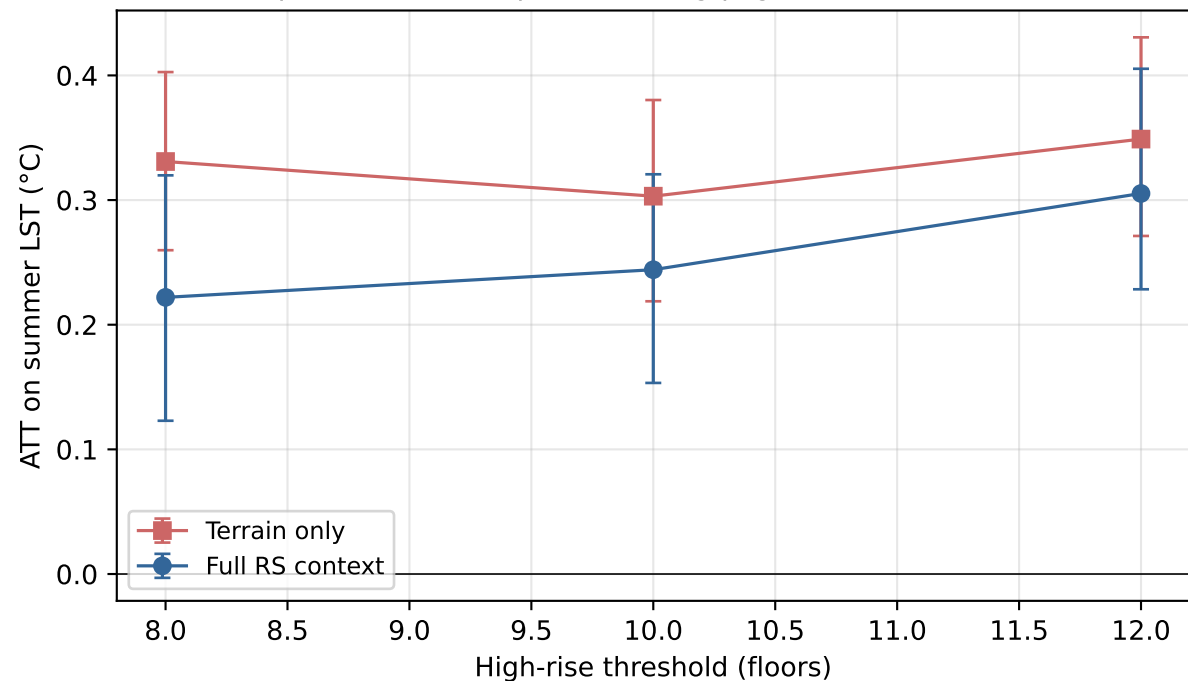
Threshold-placebo dose-response (Chongqing UHI, full vs. terrain variants)
