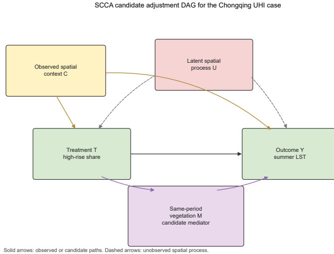
Figure 1: Candidate adjustment DAG for the Chongqing UHI case. Terrain and historical land-use are observed common causes of treatment T (high-rise) and outcome Y (summer LST). A latent spatial process U remains unobserved; SCCA reports residual Moran’s I and spatial-lag sensitivity as diagnostics for the resulting bias rather than identifying U . NDVI is shown explicitly as a possible post-treatment mediator: SCCA’s variable-role layer requires the analyst to declare whether it is added as confounder or omitted as descendant of T .
