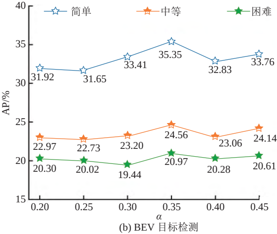
图 3 深度误差加权损失中目标检测精度随超参数的变化 Fig.3 Variation of object detection accuracy with hyper-parameters in depth error weighted loss
